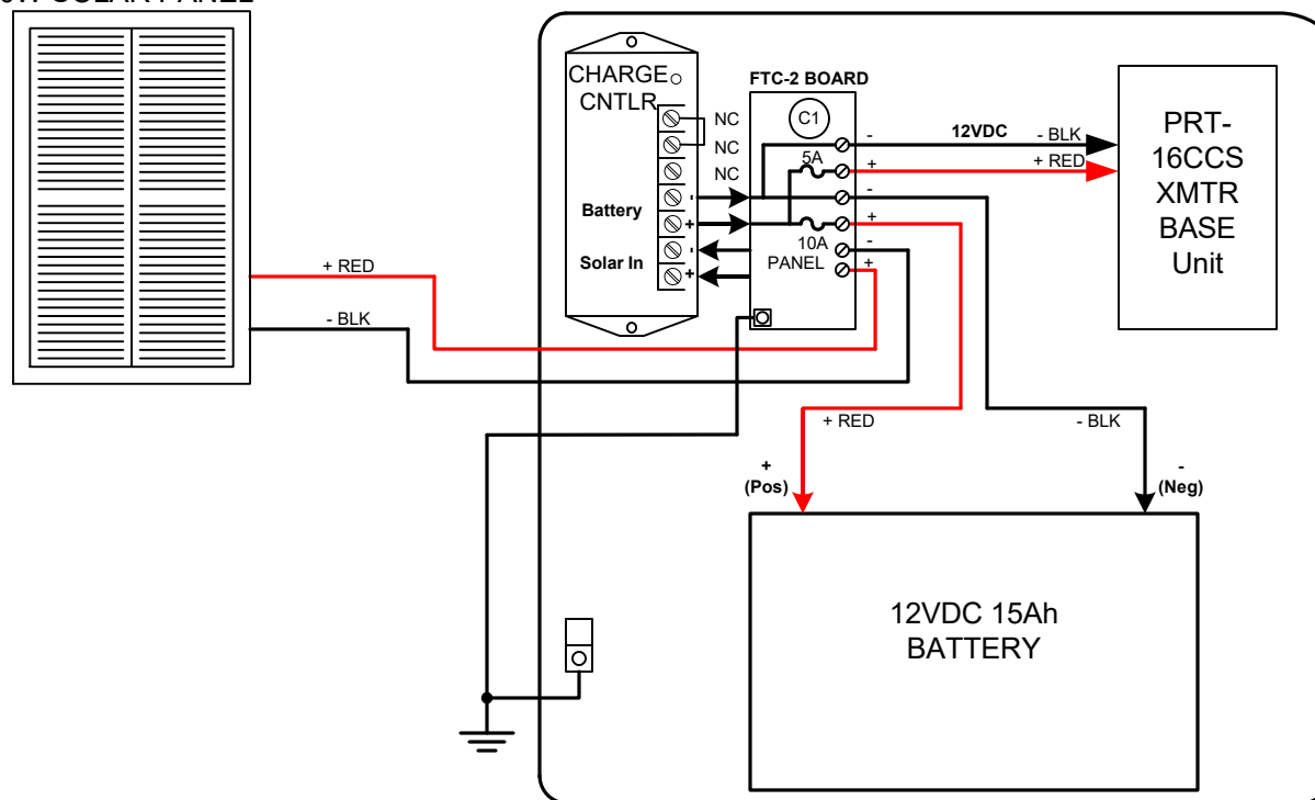
20W SOLAR PANEL
