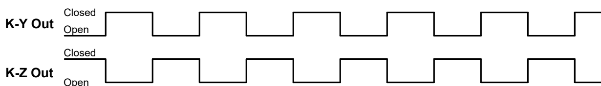
Figure 1: 2-Wire or 3-Wire TOGGLE Output Operation
