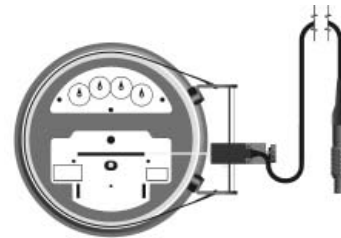
RR-DS/f Meter Disk Sensor (field mount version)
