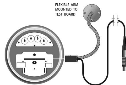
RR-DS/s Meter Disk Sensor (shop mount version)
