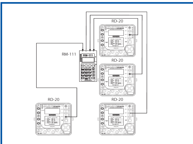
Testing Three Reference Standards
