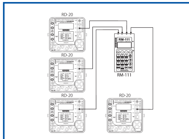
Testing a Standard Using Three Averaged Reference Standards
